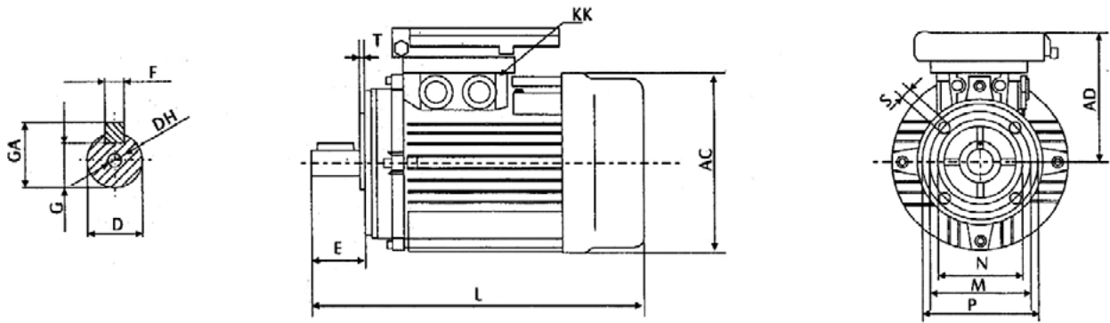
Flange Specification: B14
