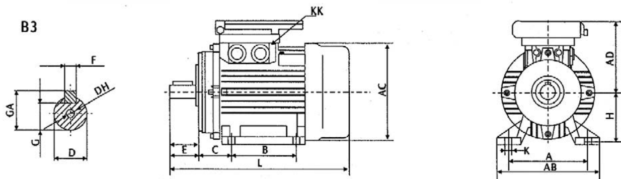
Flange Specification: B3
